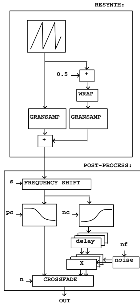
Figure 3: Overlap-add arrangement of two GRANSAMP modules, followed by the post-processing step.
