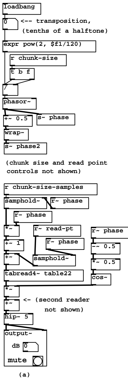
Figure 2.16: (a) two overlapped looping samplers (B10.sampler.overlap.pd); (b) the same, but with a phasor-controlled read point (B11.sampler.rockafella.pd).
